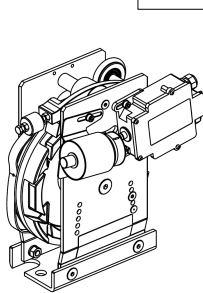
Fig. 3 Overspeed governor type R5 / R5S / R6 with remote control. Other support possible.
