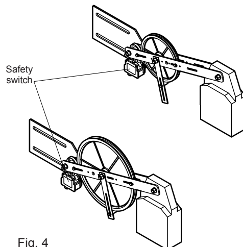
Fig. 4 Tension weight with horizontal counterweight complete with safety switch
